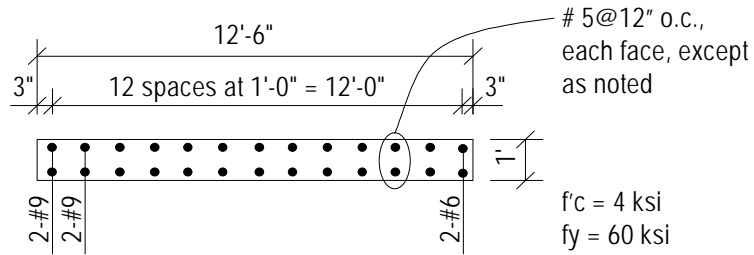
Figure 3-7: Example Two-Dimensional Wall Pier With Unsymmetrical Reinforcing
