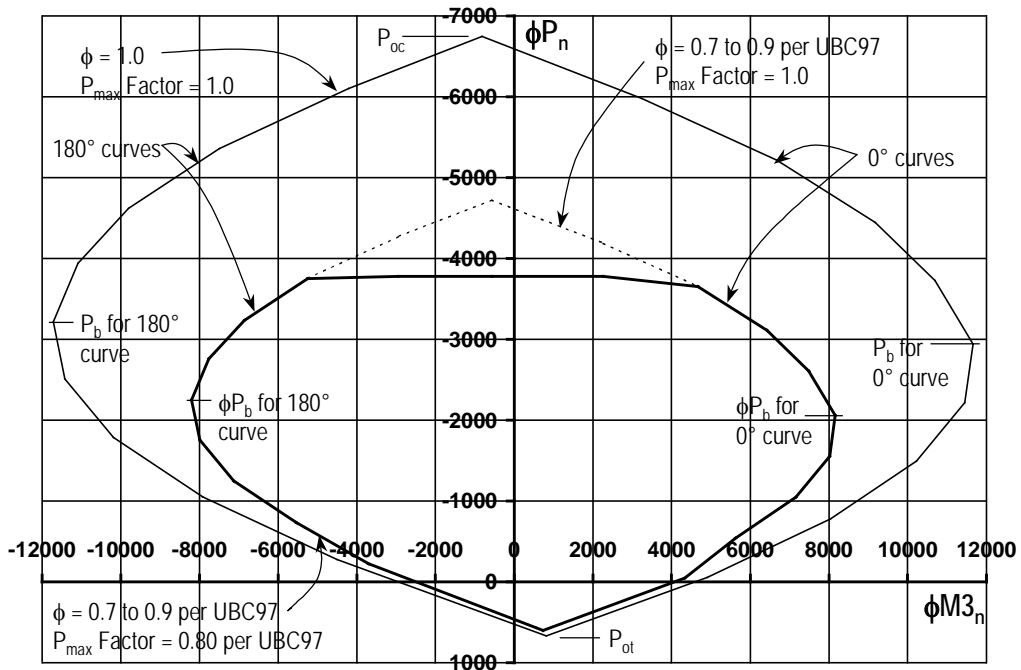
Figure 3-8 : Interaction Curves for Example Wall Pier Shown in Figure 3-7
